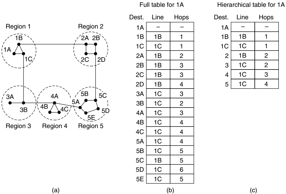
Figure 5-14. Hierarchical routing.
