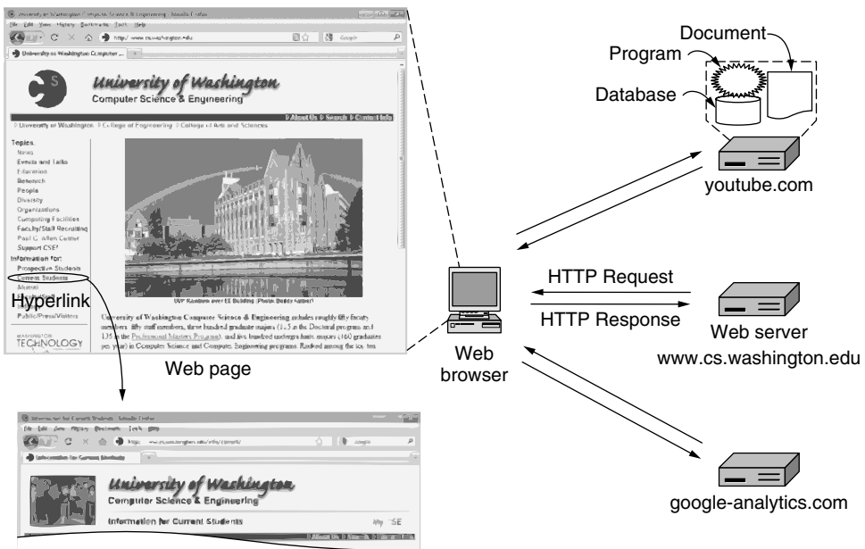
Figure 7-18. Architecture of the Web.
