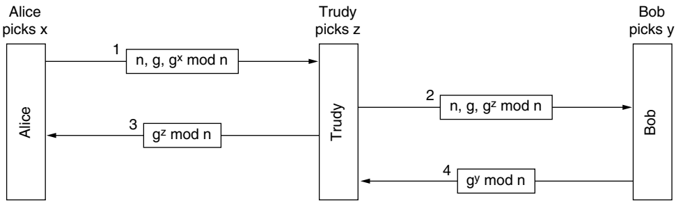
Figure 8-38. The man-in-the-middle attack.
