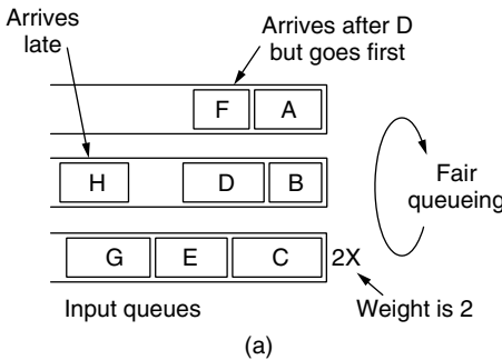
Figure 5-31. (a) Weighted Fair Queuing. (b) Finishing times for the packets.
